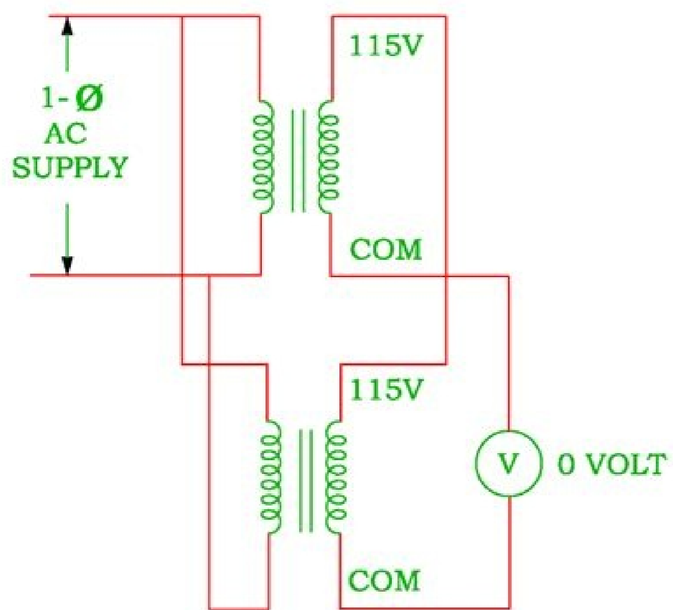
( a ) CORRECT POLARITY
