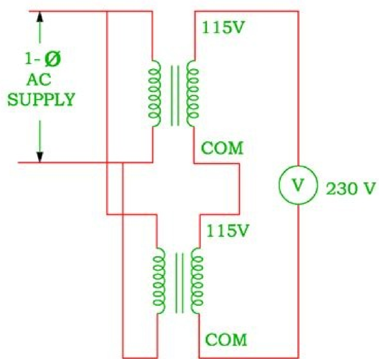
( b ) INCORRECT POLARITY
